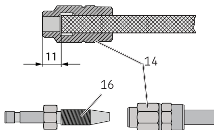
Mounting of screw sleeves and hose studs Fig. 24
