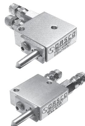
Spray Nozzle - SWN LP, Side Connections Spray Nozzle - SWN IP, Back Connections
